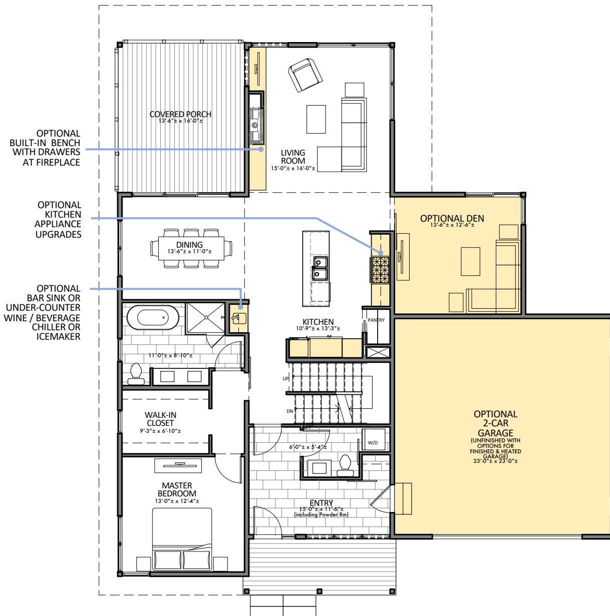
FIRST FLOOR PLAN with OPTIONAL DEN, 2-CAR GARAGE, BUILT-INS. and APPLIANCE UPGRADES 1,593 SF (EXCLUDING GARAGE)
